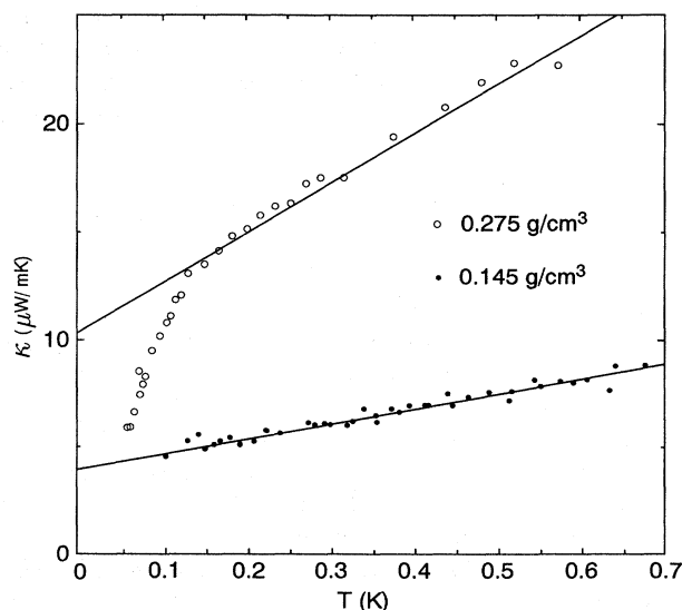
FIG. 36. \kappa(T) between 0.05 and 0.7 \text{ K} . The solid lines are fits to Eq. (8.11). After Bernasconi et al. (1992).
