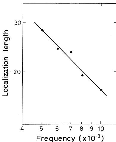
FIG. 16. Values of localization length \Lambda(\omega) plotted as a function of frequency on a log-log scale. The straight line [\Lambda(\omega) \propto \omega^{-0.71}] drawn using least-squares fitting shows that fractons in the ensemble follow the correct fracton dispersion law. After Yakubo and Nakayama (1989a).
